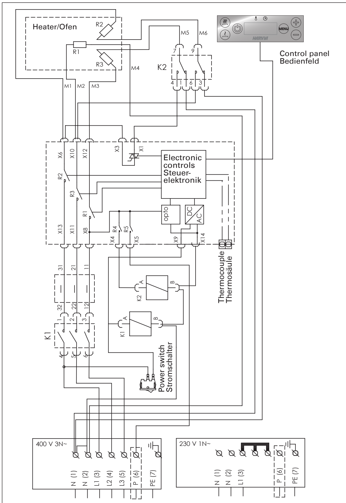
Figure 12. Electrical connections of heater Abbildung 12. Elektroanschlüsse der Saunaöfen
