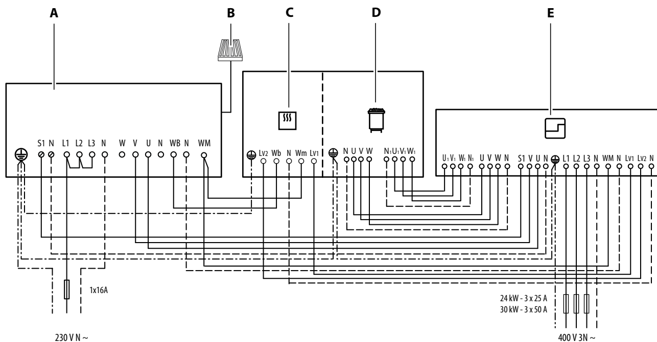
EOS Herkules XL S120 Vapor HD 24 kW terminal diagram
