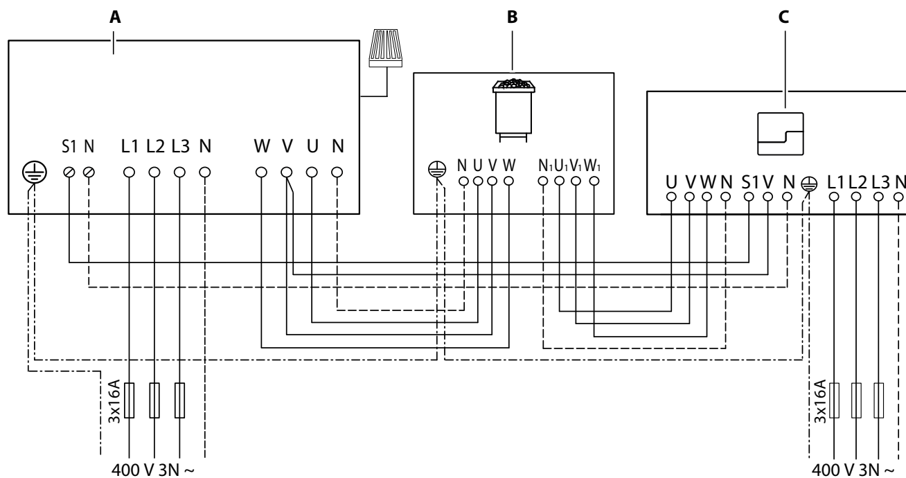
EOS Herkules XL S120 HD 18 kW terminal diagram
